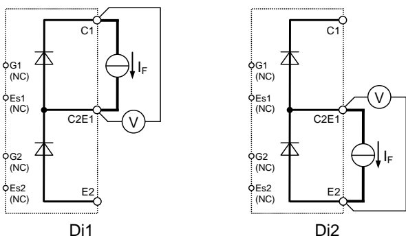
V_F test circuit
