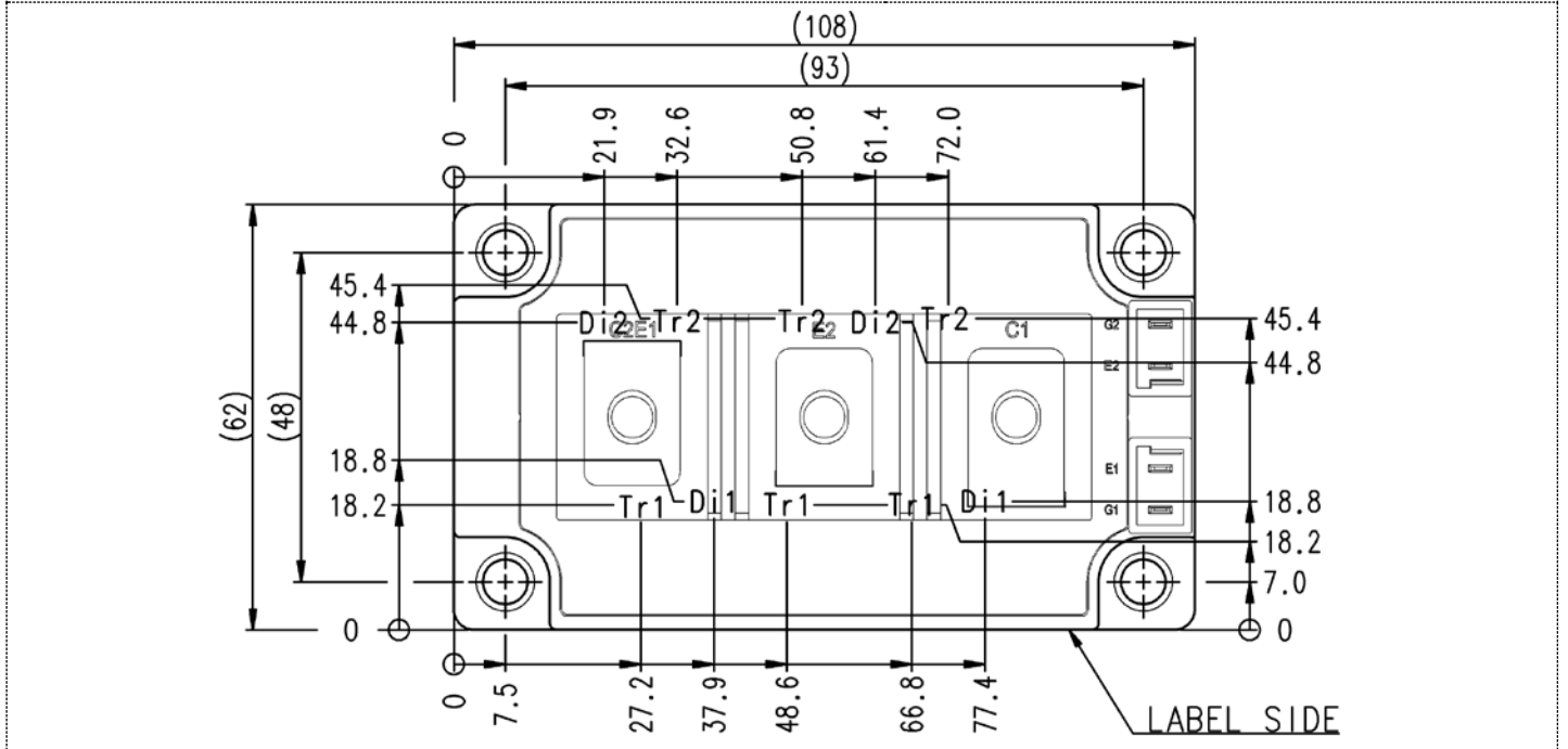
Tr1/Tr2: IGBT, Di1/Di2: FWD
