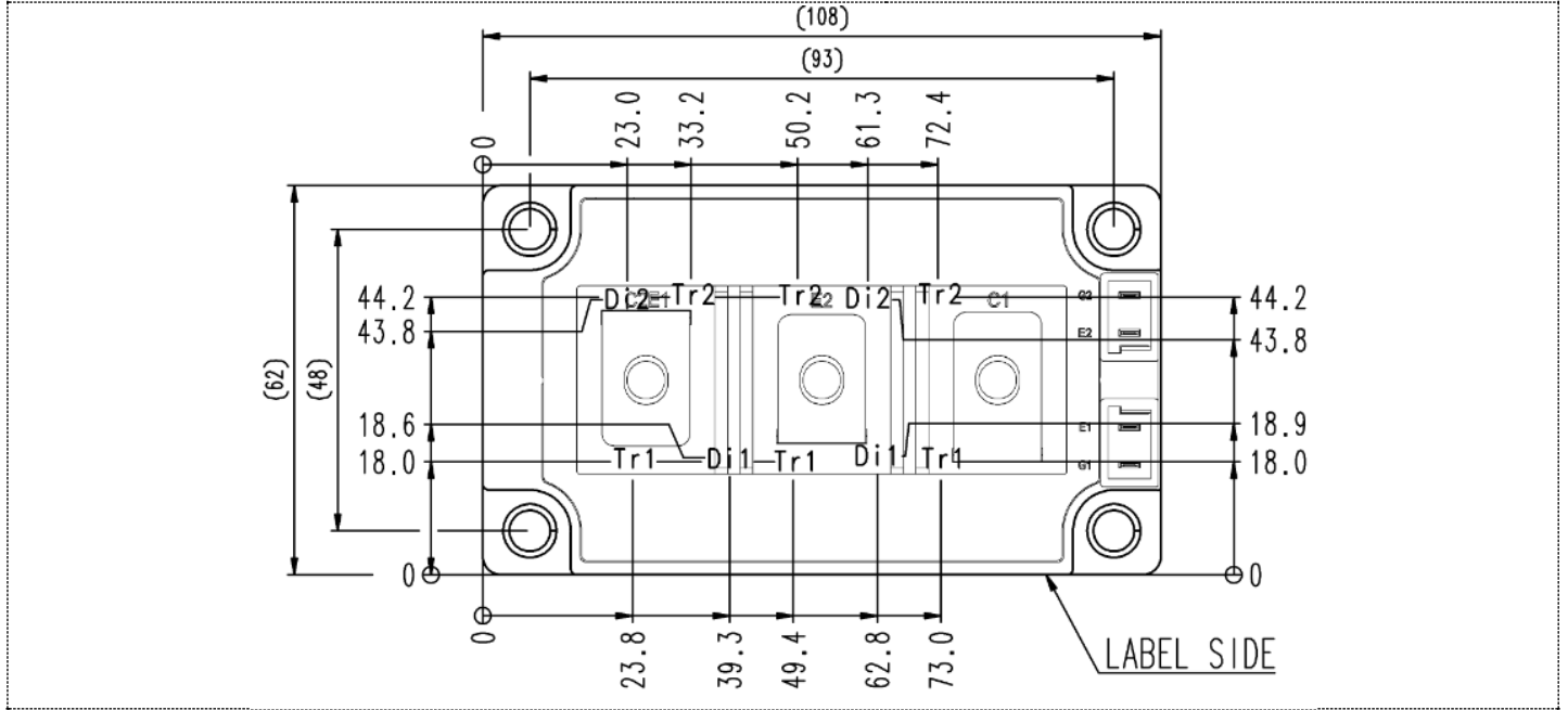
Tr1/Tr2: IGBT, Di1/Di2: FWD
