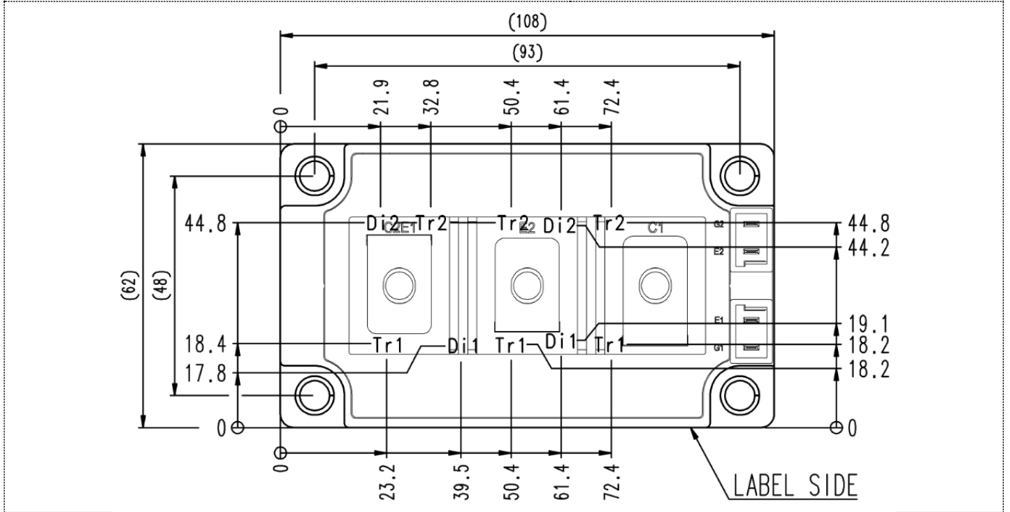
Tr1/Tr2: IGBT, Di1/Di2: FWD
