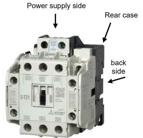
Fig1: Product Appearance (S-T21)
