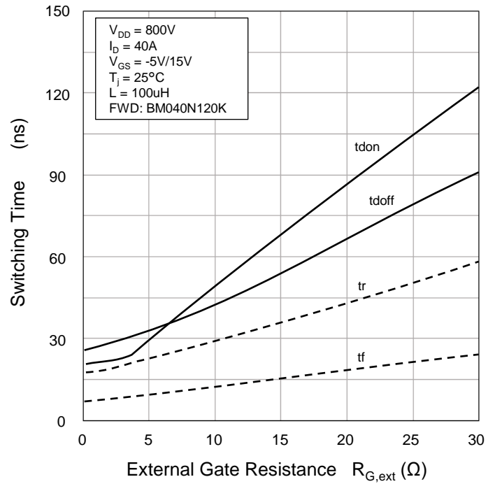
Figure 14 Typical Switching Times vs. R_{G,ext} ( T_j = 25^\circ\text{C} )
